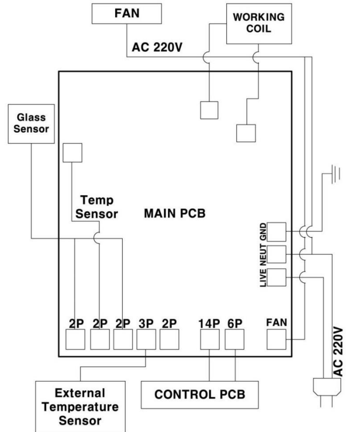
DCP23 Wiring Diagram
