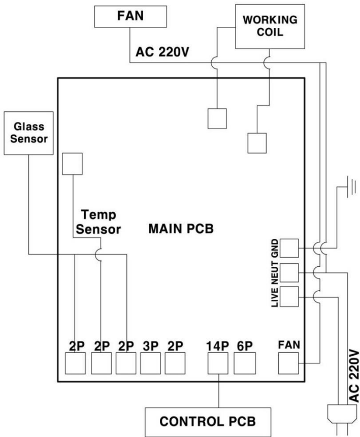
DCR23/DWR04 Wiring Diagram
